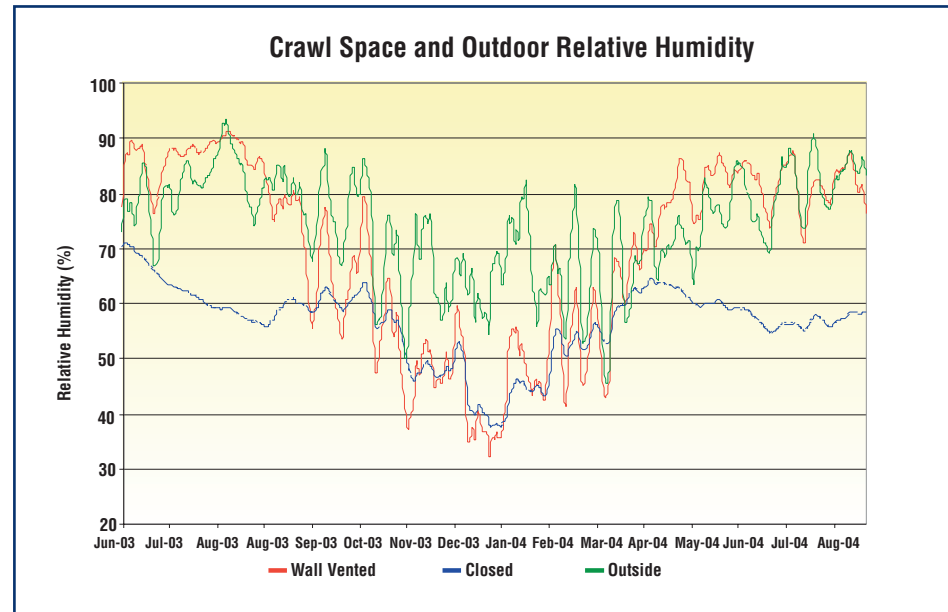
Summer (June-August) Relative Humidity Summary
