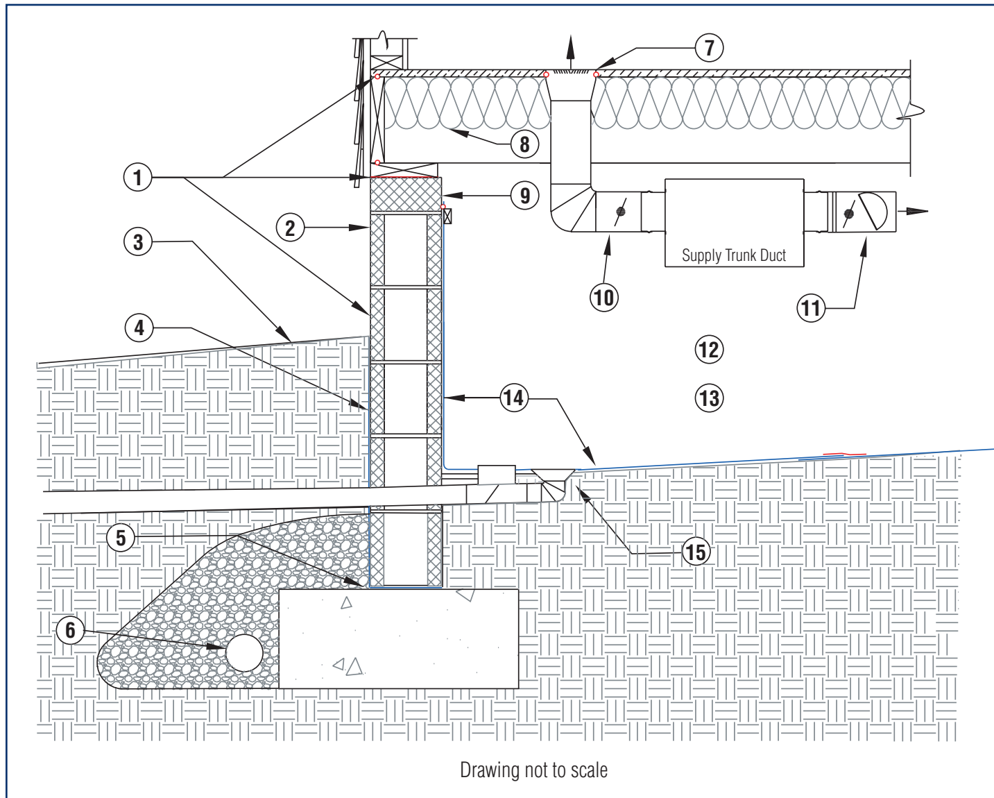
Advanced Energy Sample Design: A Closed Crawl Space With Supply Air and Floor Insulation
