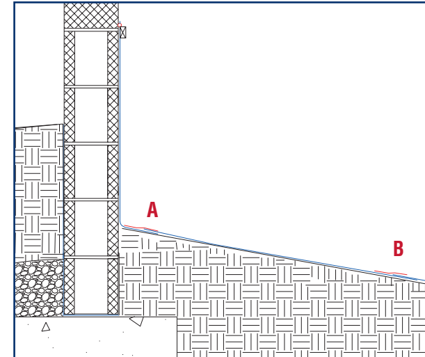
Overlap seams in the vapor retarder material to reduce the chance that liquid water running downhill from the wall or ground will collect against the underside of the sealed seams. Lap the ground vapor retarder on top of the wall vapor retarder (A) and lap downhill sections of vapor retarder over uphill sections of vapor retarder (B).
