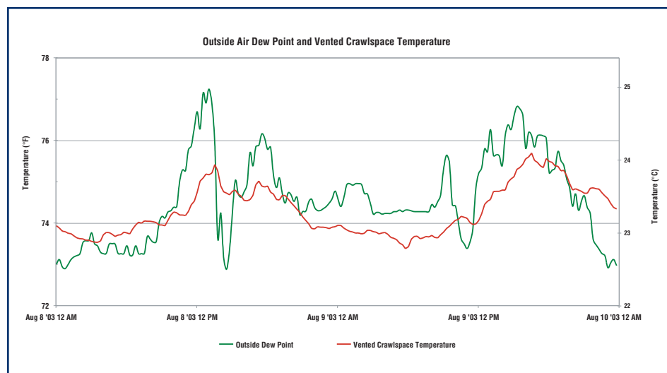
This data from the Princeville site shows that for most of a very humid 48-hour period, the outside dew point exceeds 74° F (24° C) and is higher than the temperature inside the crawl space. If this outside air enters the crawl space, the water vapor will condense on surfaces inside. Note that this was not a period of very rainy weather; records indicate only 0.2 inches of rainfall over this entire 48-hour period.
