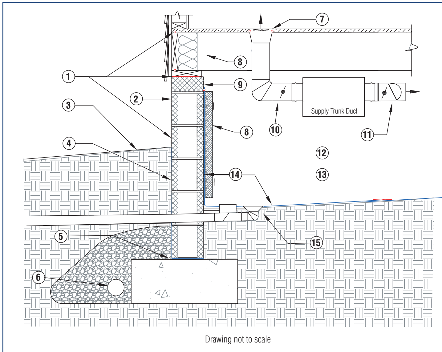
Advanced Energy Sample Design: A Closed Crawl Space With Supply Air and Wall Insulation
